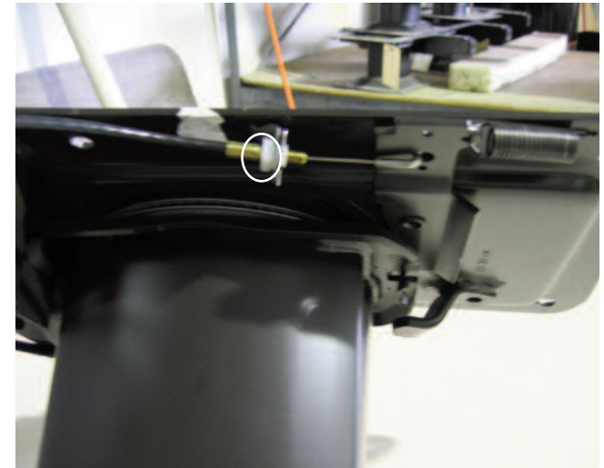
Step 6 If needed Nylon Nut can be turned to increase or decrease tension
