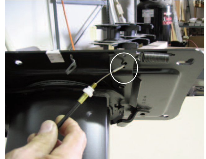
Step 2 Insert end of cable into round hole on swivel release arm
