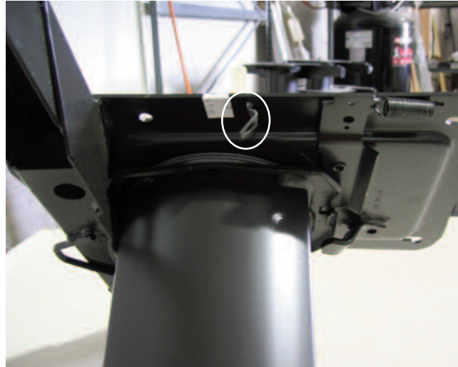
Step 1 insert bracket in slotted hole on underside of top plate
